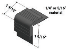
VCD-XX 1/4" or 5/16" material on step and riser
